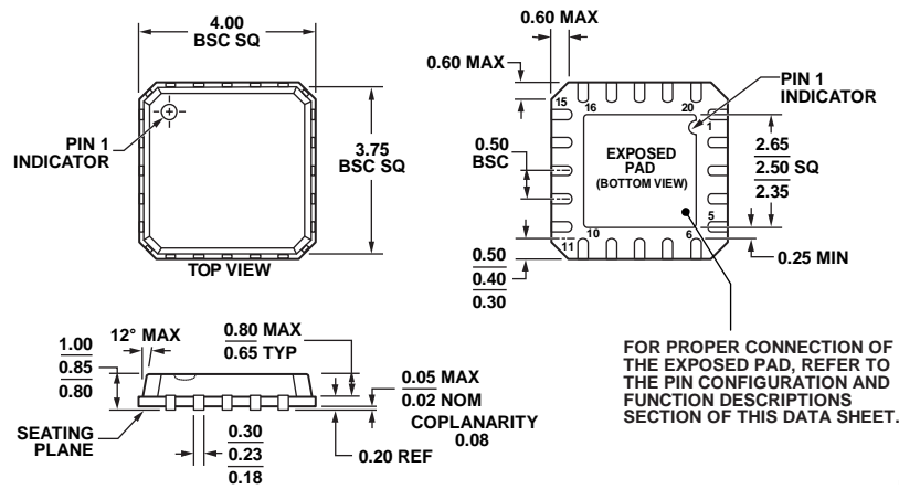
Figure 22. 20-Lead Lead Frame Chip Scale Package (LFCSP_VQ) 4 mm × 4 mm Body, Very Thin Quad (CP-20-4) Dimensions shown in millimeters
